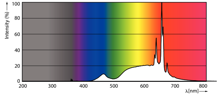
Spectral Power Distribution Colour - MAS LED spot VLE D 2.8-35W GU10 927 36D
