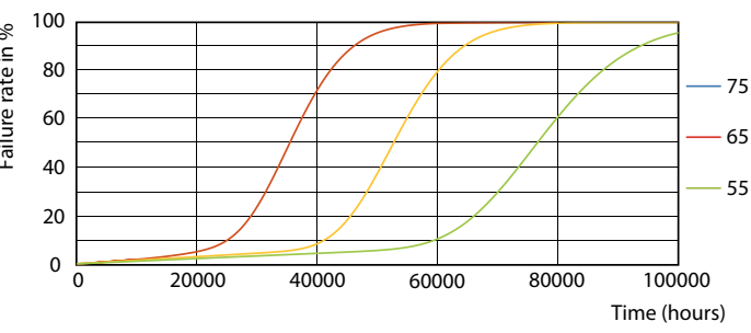
FailureRate
